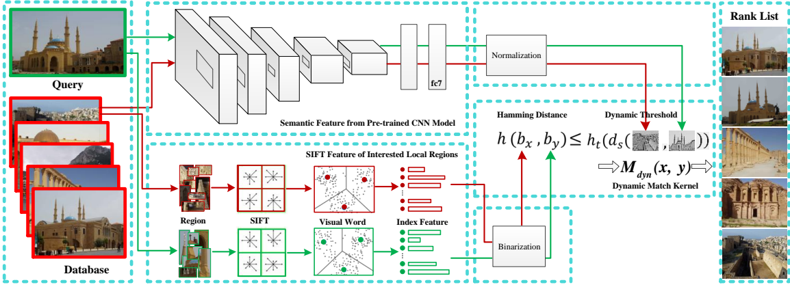
Fig. 3. Main steps of the proposed semantic-constrained image retrieval algorithm. Different from prior work based on local descriptors with static match kernels, we calculate an adaptive threshold h_t(d_s) using a pre-trained CNN to construct the dynamic match kernel. The proposed dynamic match kernel function is shown in Eq. 6 where h(b_x, b_y) and h_t(d_s) are computed with local invariant features and deep features, respectively.
