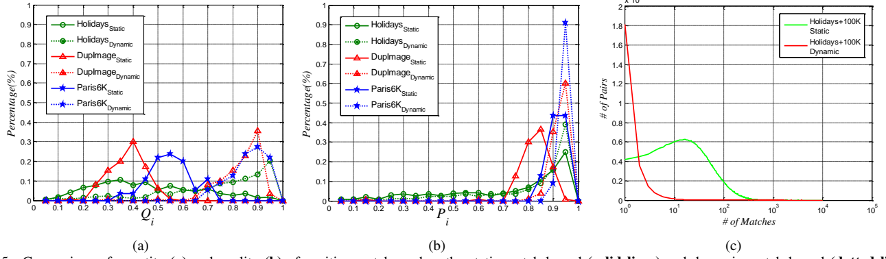
Fig. 5. Comparison of quantity (a) and quality (b) of positive matches when the static match kernel (solid lines) and dynamic match kernel (dotted lines) are applied on three benchmarks (The curves of other two datasets are similar). Q_i and P_i are defined in Eq. 9 and Eq. 10, respectively. The vertical axes in both figures represent the percentages of feature matches falling into the corresponding quantity and quality bins. (c) shows the statistics of the non-zero matches between image pairs in Holidays dataset with 100K distractors. The horizontal axis indicates the number of matches, and the vertical axis represents the number of image pairs which have the corresponding match number. More details can be found in Section III-D.
