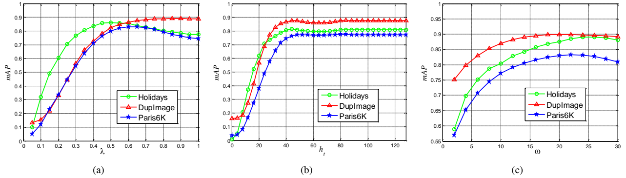
Fig. 6. Parameter analysis on Holidays, Paris6K and DupImage datasets. (a) Effect of the parameter \lambda which linearly scales the dynamic threshold in Eq. 5. We set \lambda = 0.6 since it leads to the best performance. (b) The mAP of the static match kernel against the fixed threshold h_t in Eq. 2. The mAP tends to be stable when h_t > 40 , where detailed analysis of \lambda and h_t can be found in Section IV-B. (c) Influence of the parameter \omega in Section IV-F which controls the intensity of the exponent when the dynamic selective match function [51] is applied instead of the dynamic threshold. We set \omega = 22 in this paper.
