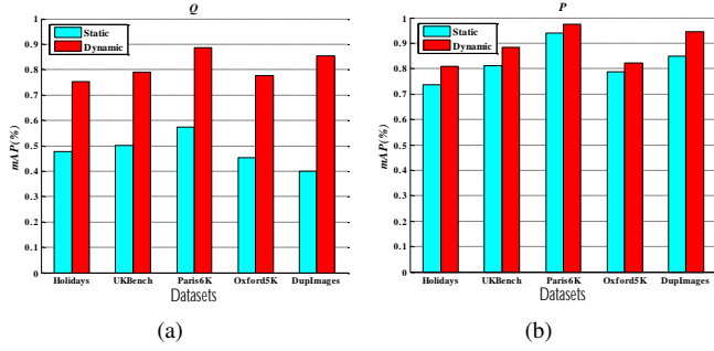
Fig. 4. Comparison between the static and dynamic match kernels in terms of quantity and quality scores, where Q and P measures the quantity and quality of positive matches, respectively.
